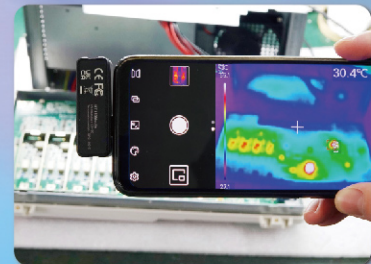
PCBA Inspection
