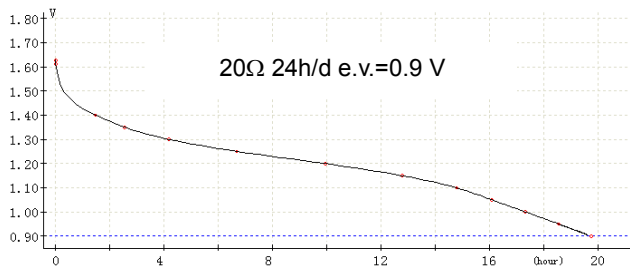
Chart 1. Discharge diagram
